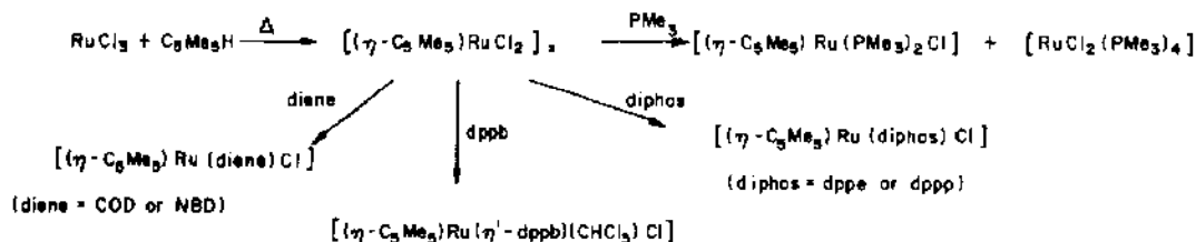
Scheme 49.
