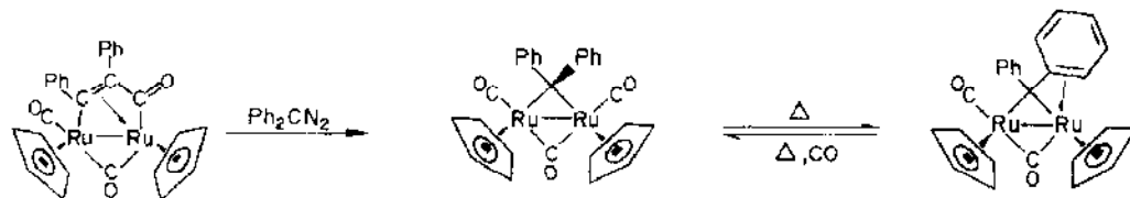
Scheme 62.
