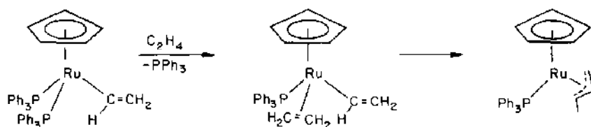
Scheme 33.
