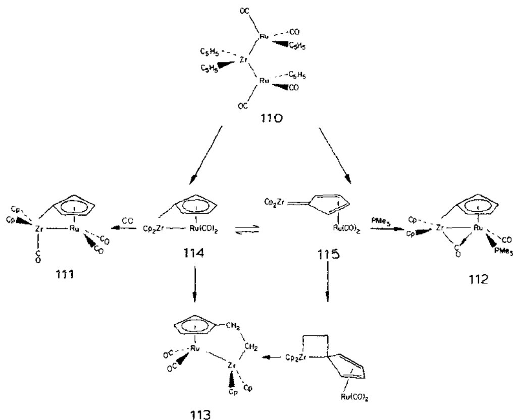
Scheme 81.
