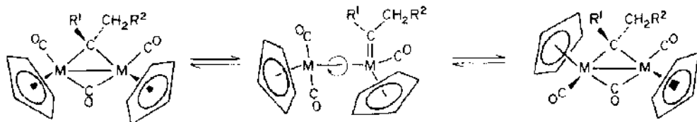
Scheme 57.
