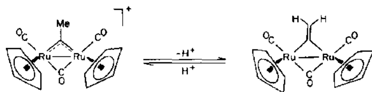
Scheme 67.
