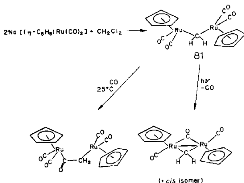
Scheme 70.
