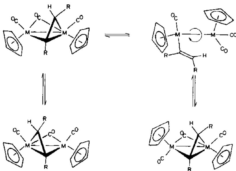
Scheme 56.
