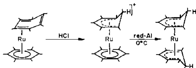
Scheme 10.
