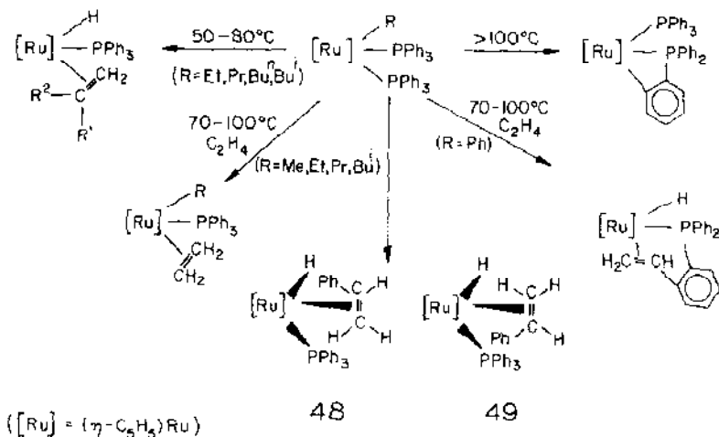
Scheme 32.
