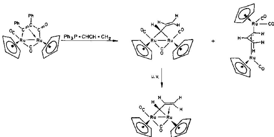
Scheme 60.
