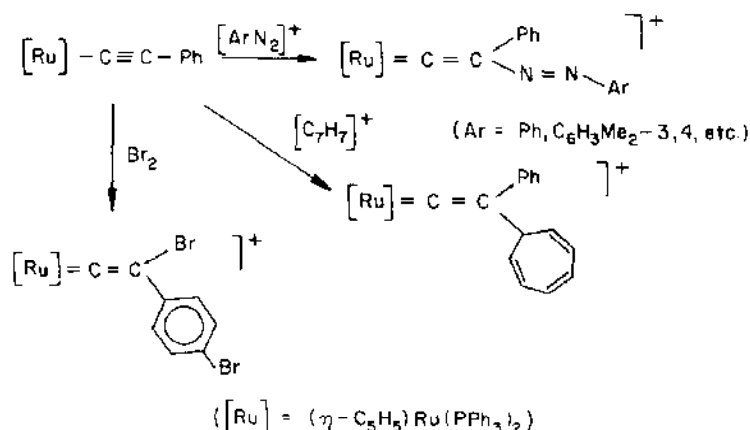
Scheme 36.
