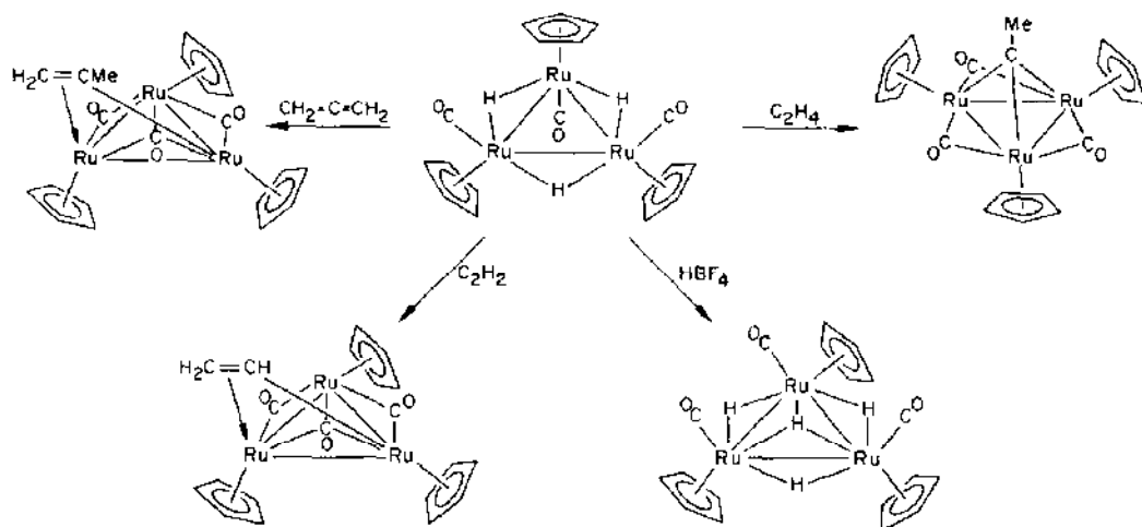
Scheme 78.
