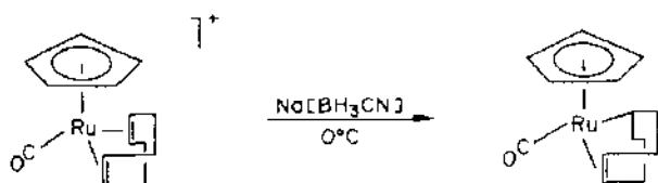
Scheme 43.
