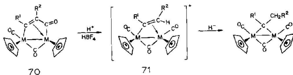
Scheme 55.
