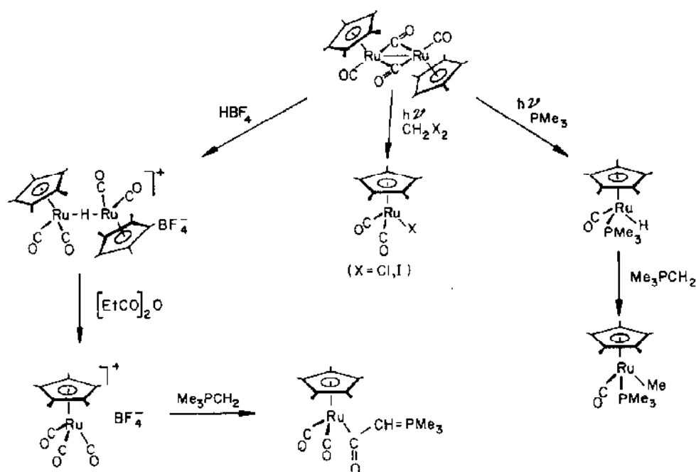
Scheme 71.
