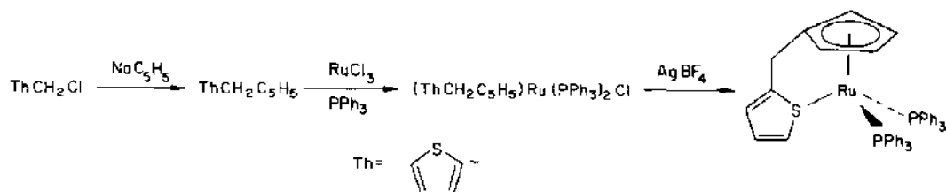
Scheme 48.
