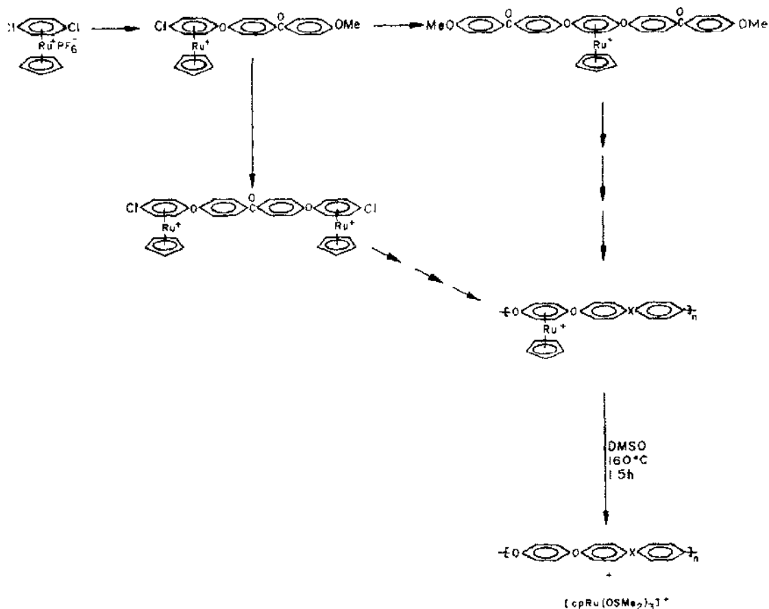
Scheme 47.
