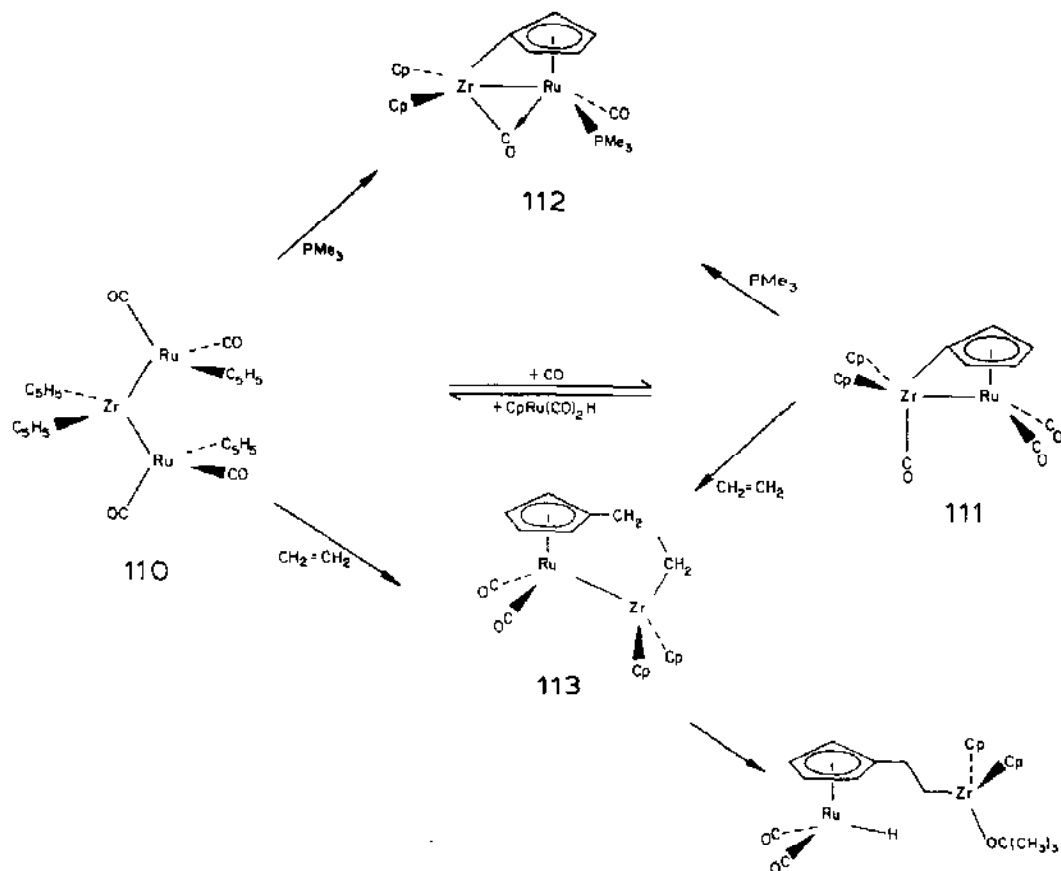
Scheme 80.
