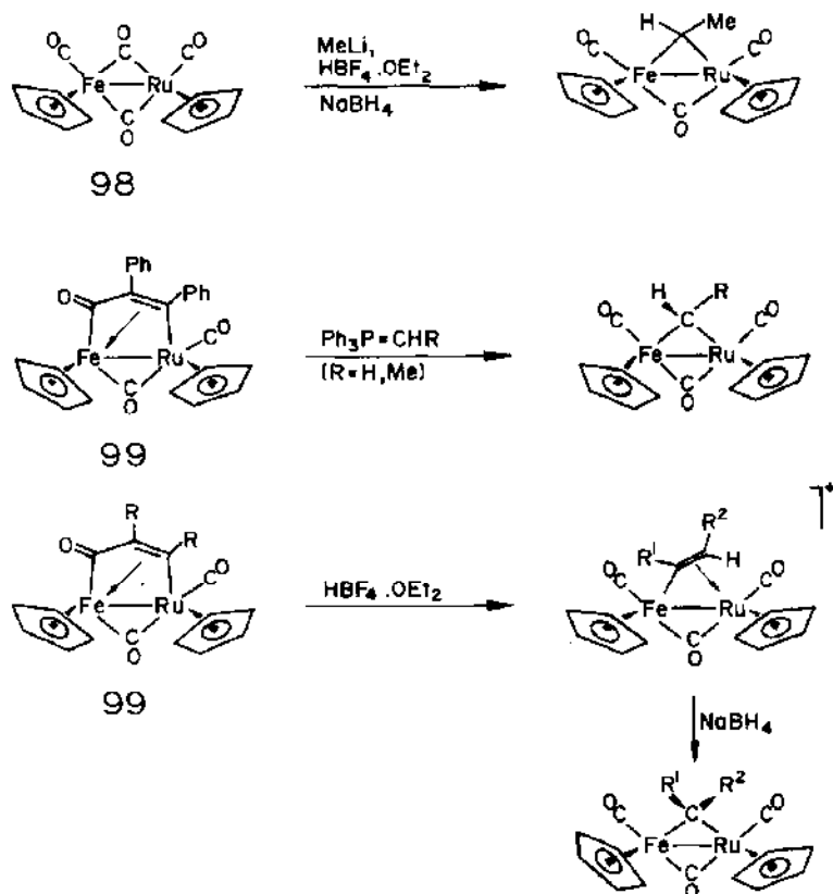
Scheme 76.
