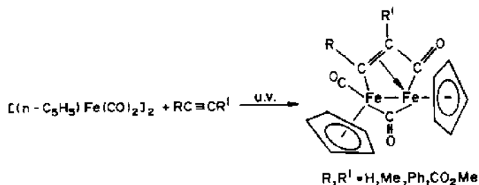
Scheme 54.
