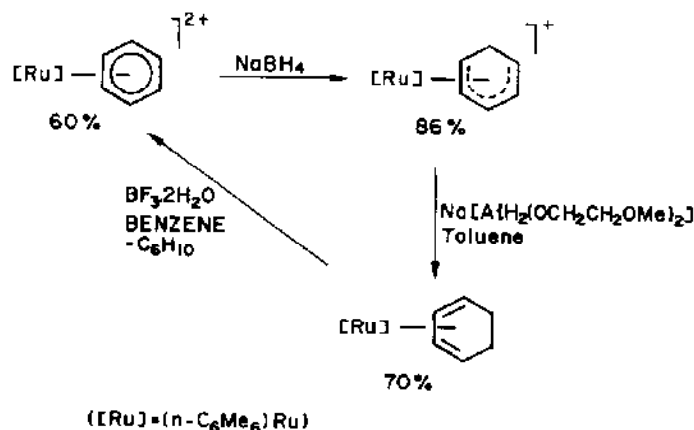
Scheme 53.
