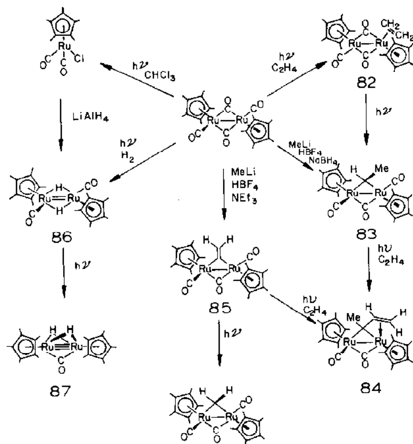
Scheme 72.
