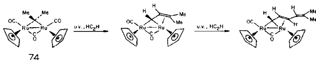
Scheme 63.
